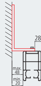
View of vertically aligned angle brackets
