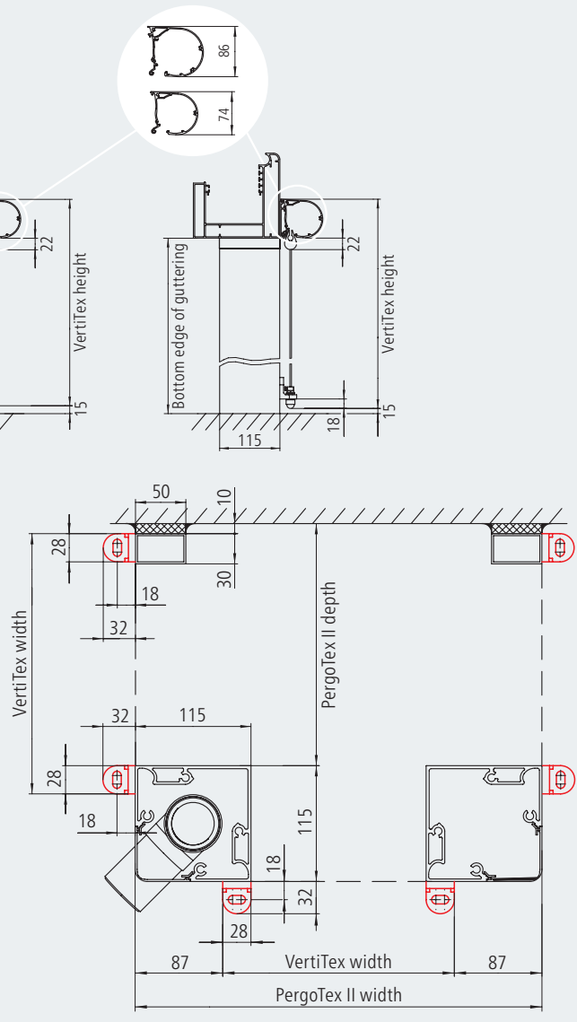
Top view of the VertiTex rope guide on the PergoTex II (front and side)
