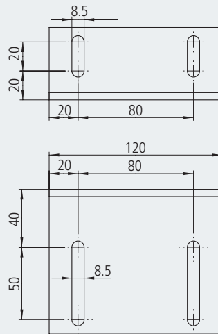
weinor PergoTex II Basic 100 x 50 x 5 x 120 mm angle bracket
