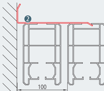
"Large" lateral wall bracket ②, for unit 2 with drive on the left (lateral spacing of 100 mm)
